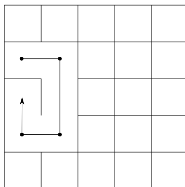
Figure 351: How the recursive backtracker algorithm works (1)
